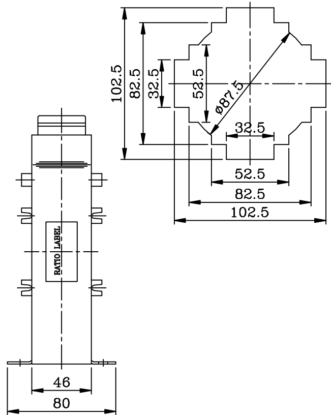
SIDE VIEW
